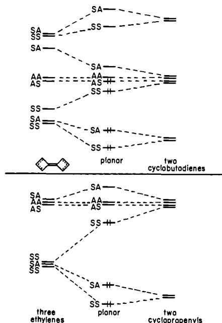
Figure 7. The energy levels of dicyclobutadiene and dicyclopropenylidene. At right are correlation diagrams relating the levels of a 90^\circ twisted molecule to those of the planar geometry. At left are interaction diagrams showing the construction of the planar from energy levels from noninteracting components.
