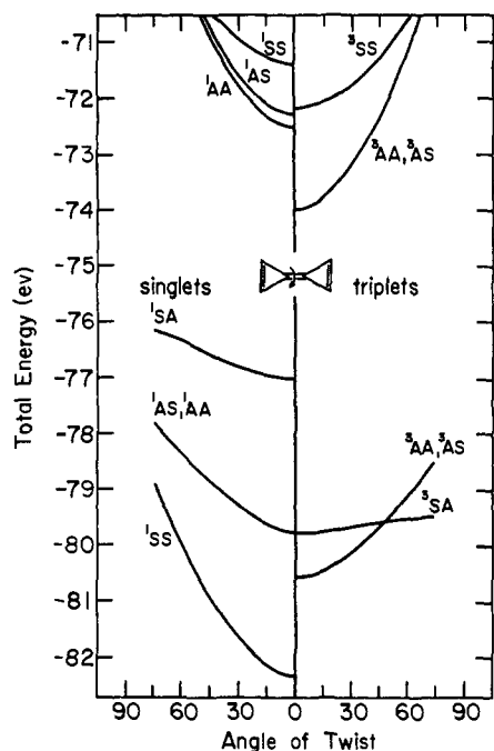
Figure 9. Total energy as a function of twist angle for the lowest singlets (left) and triplets (right) of dicyclopropenylidene. Double labels imply two energy curves nearly coincident.
