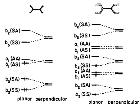
Figure 10. Correlation diagrams for bialllyl and bipentadienyl.
